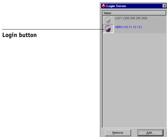
Command WorkStation
