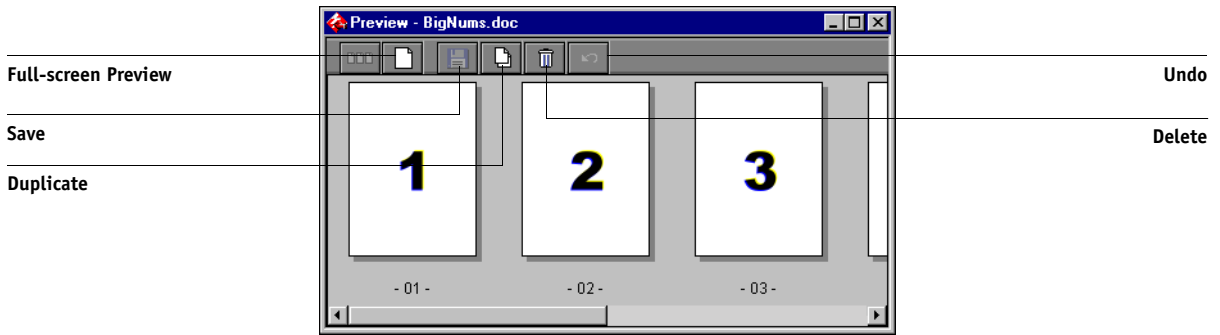
Command WorkStation
