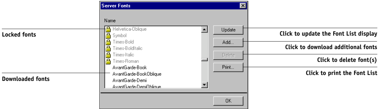
Command WorkStation
