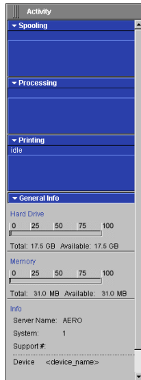
Command WorkStation
