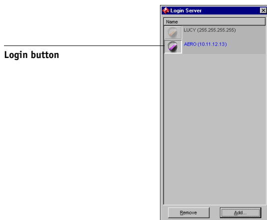
Command WorkStation
